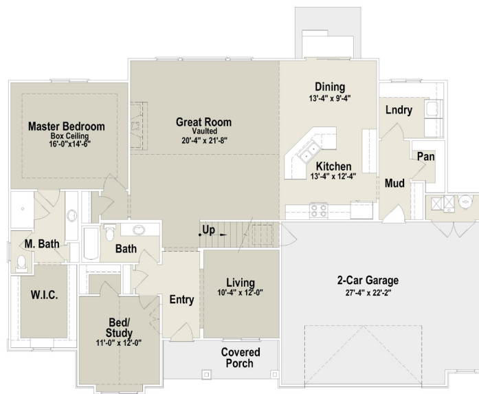
Main Floor Plan 1980 sq. ft.
