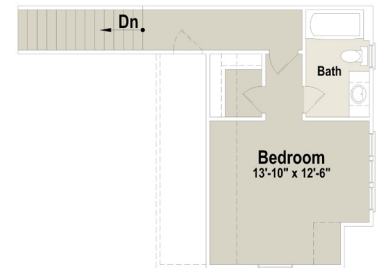
Second Floor Plan 250 sq. ft.
