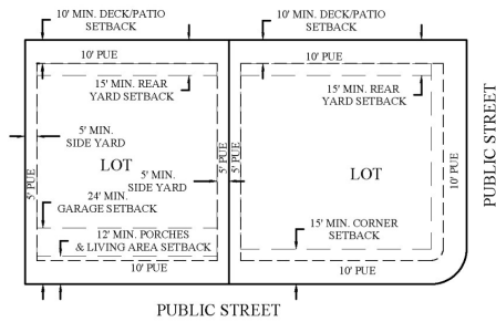
TYPICAL BUILDING SETBACKS N.T.S.
