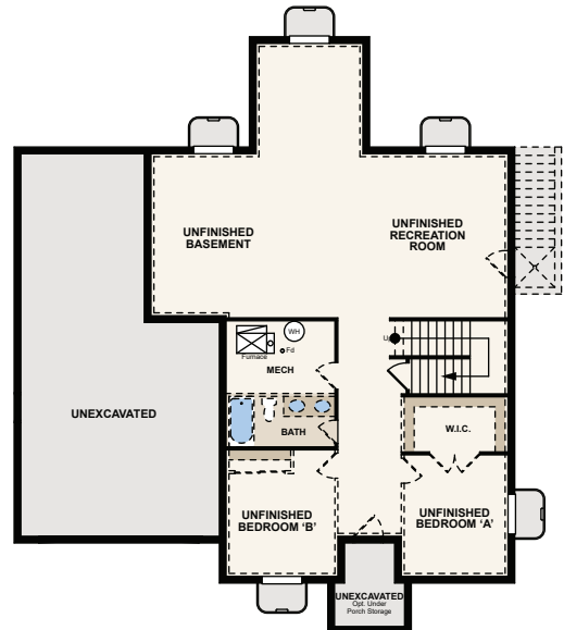
UNFINISHED BASEMENT W/SUNROOM
