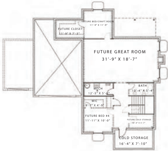
BASEMENT FLOOR
