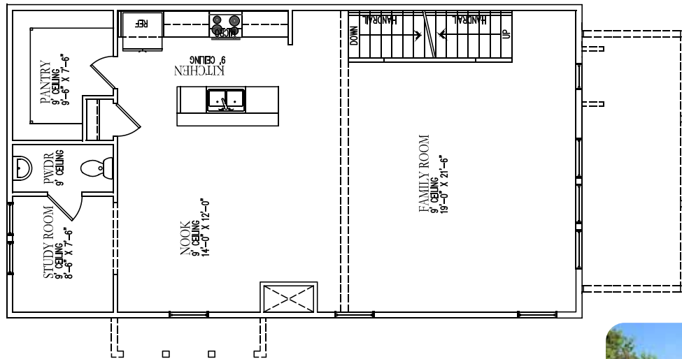
UPPER LEVEL
