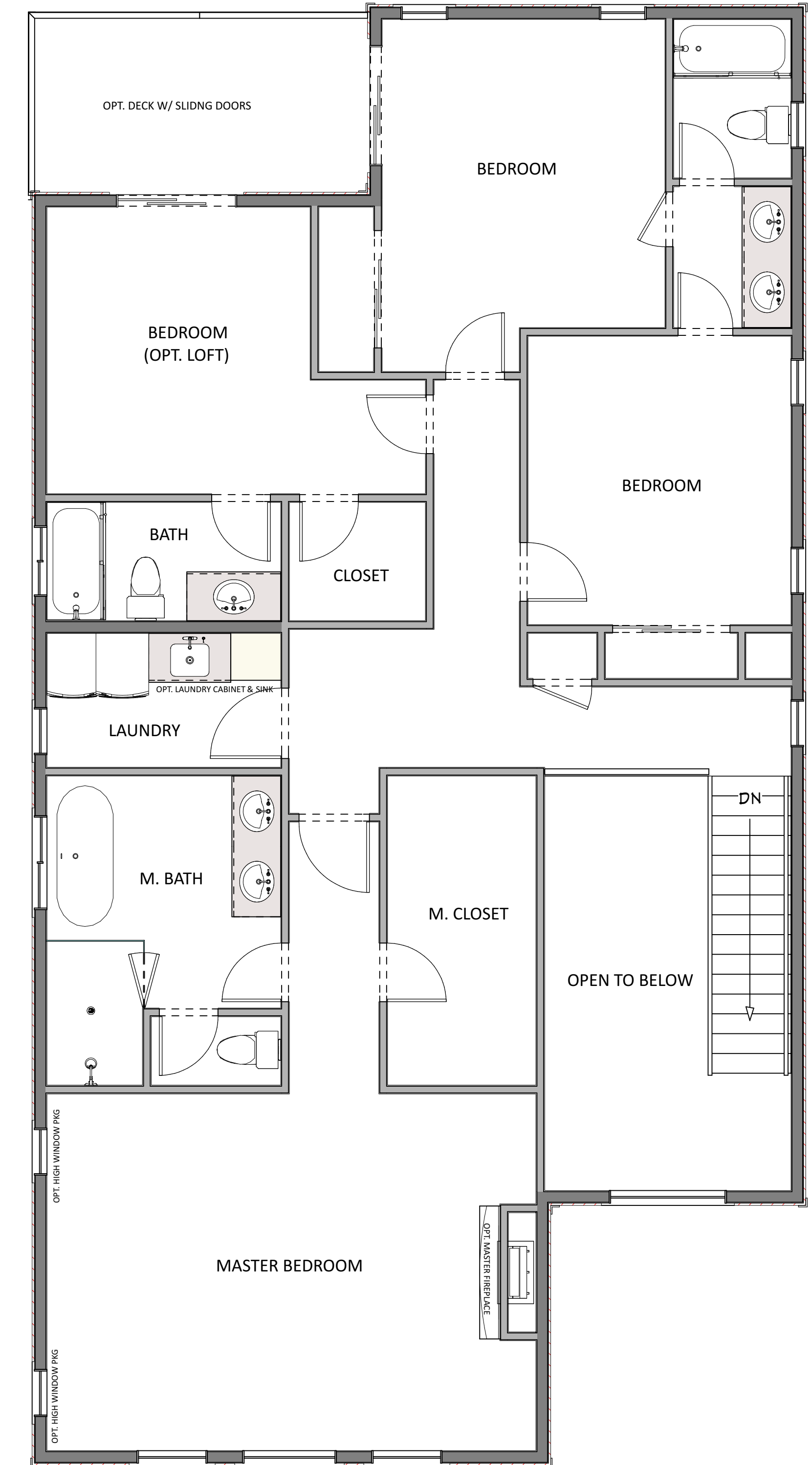
UPPER FLOOR
