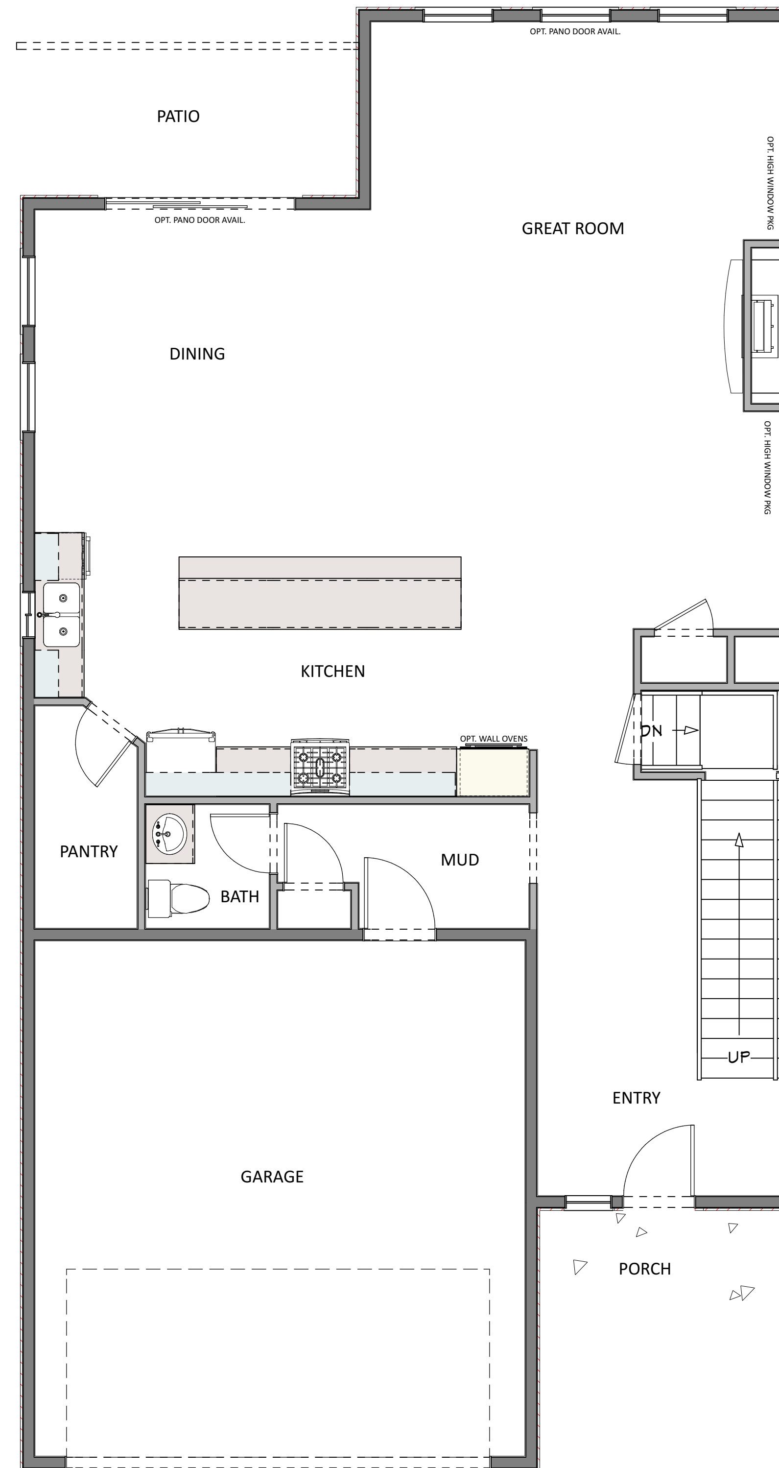
MAIN FLOOR
