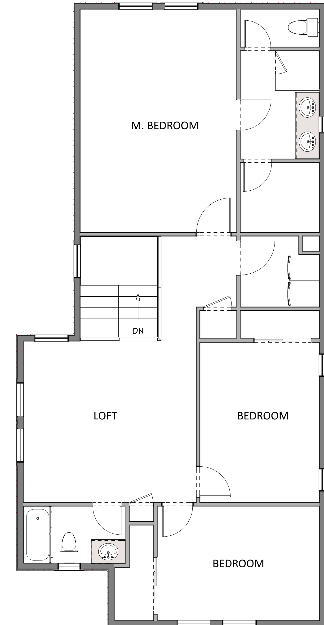
UPPER FLOOR
