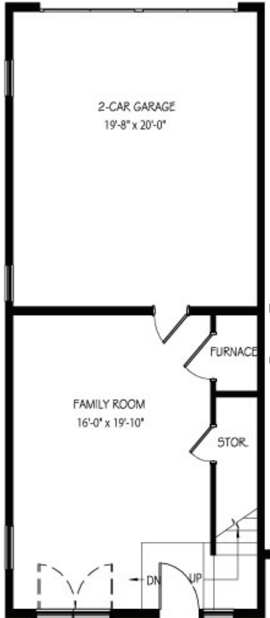
LEVEL ONE - 430 SQ FT
