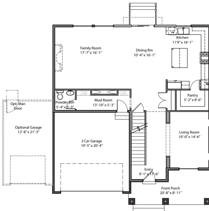
MAIN FLOOR
