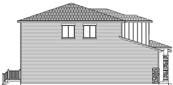
LEFT ELEVATION
