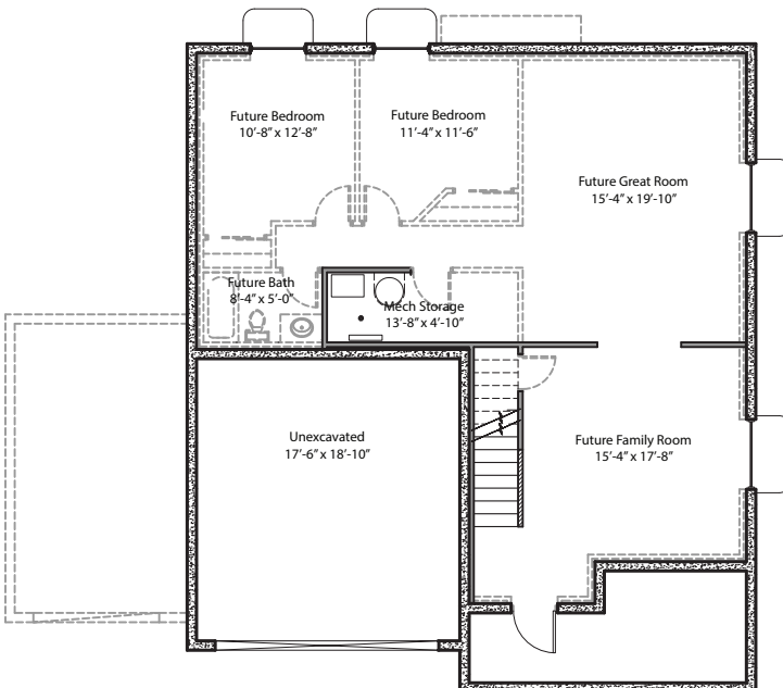
BASEMENT FLOOR
