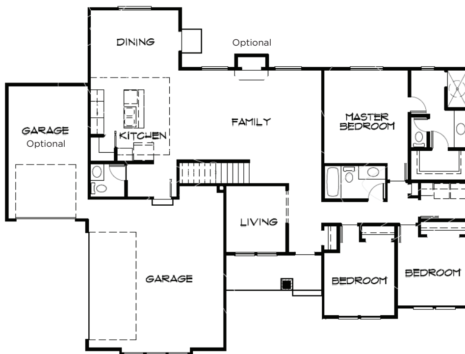
MAIN LEVEL
