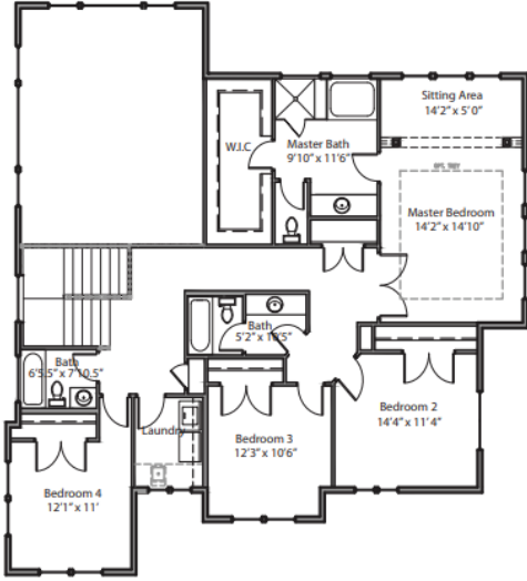
UPPER FLOOR
