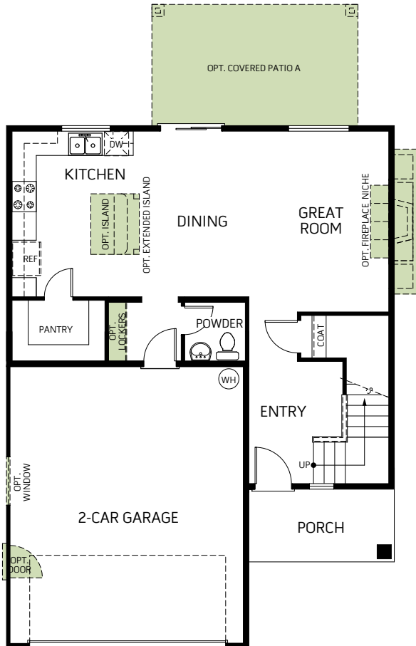
FIRST FLOOR PLAN 762 Sq. Ft.
