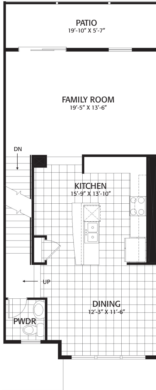
FIRST LEVEL
