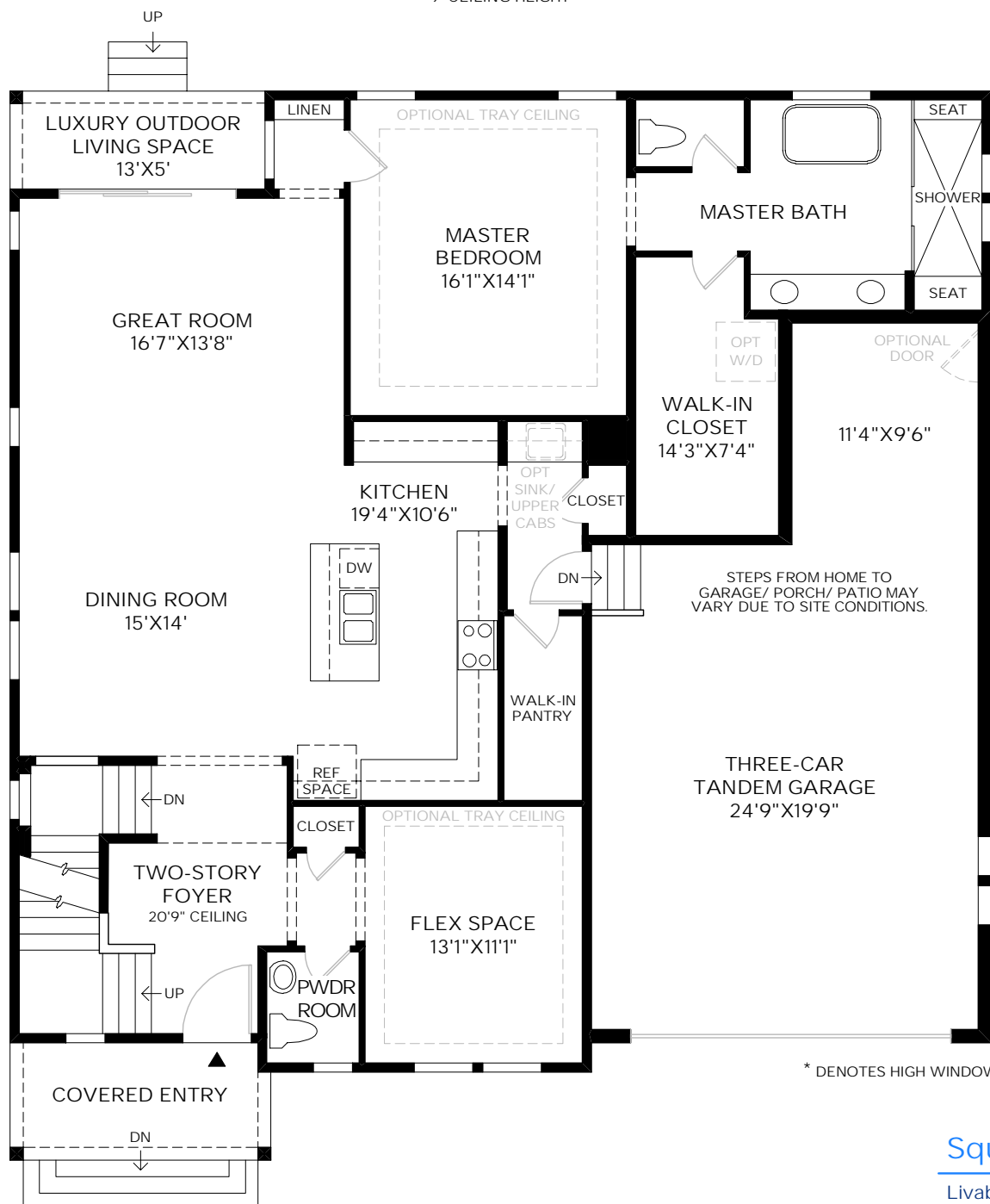
First Floor 10' CEILING HEIGHT
