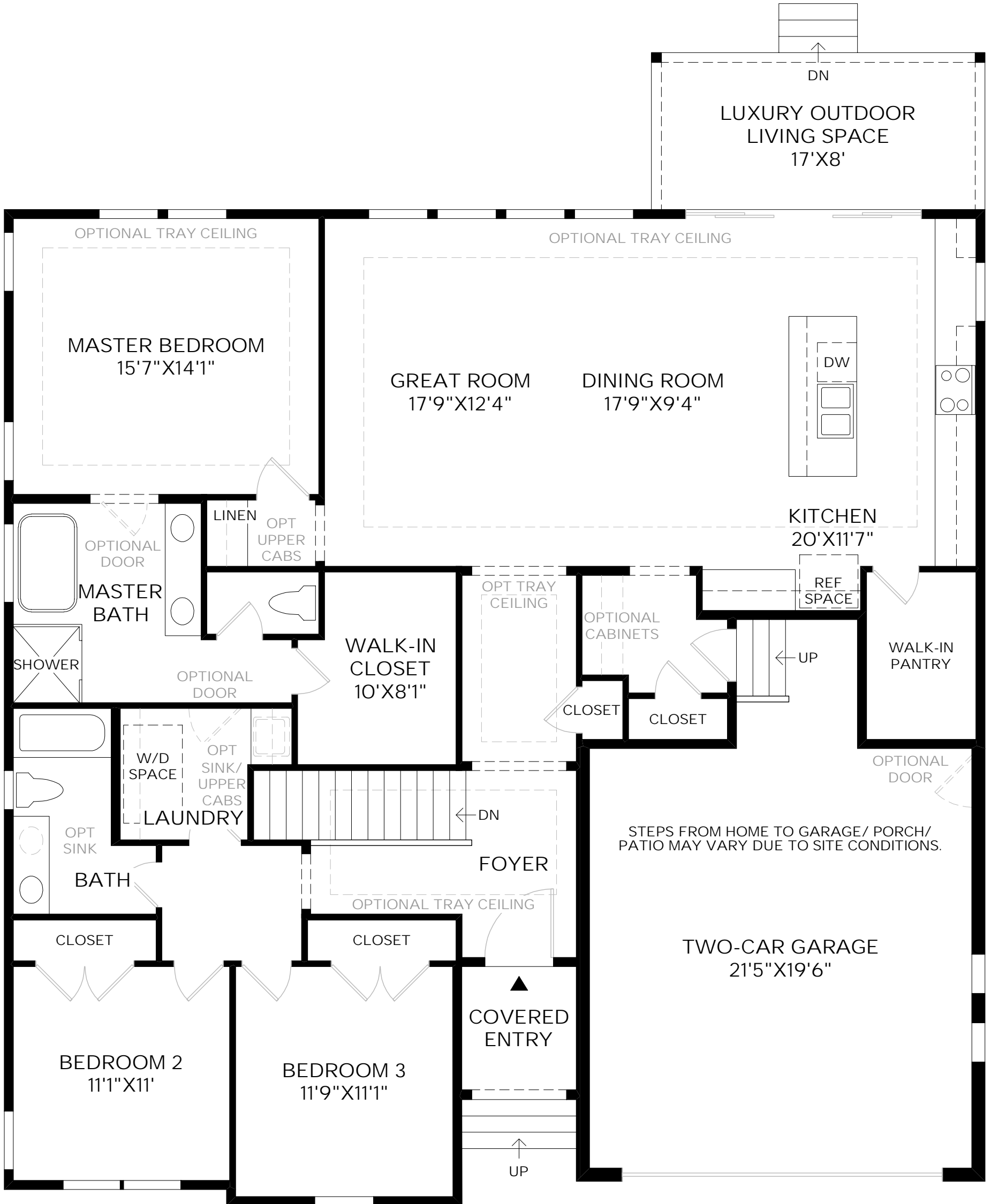
Floor Plan 10' CEILING HEIGHT
