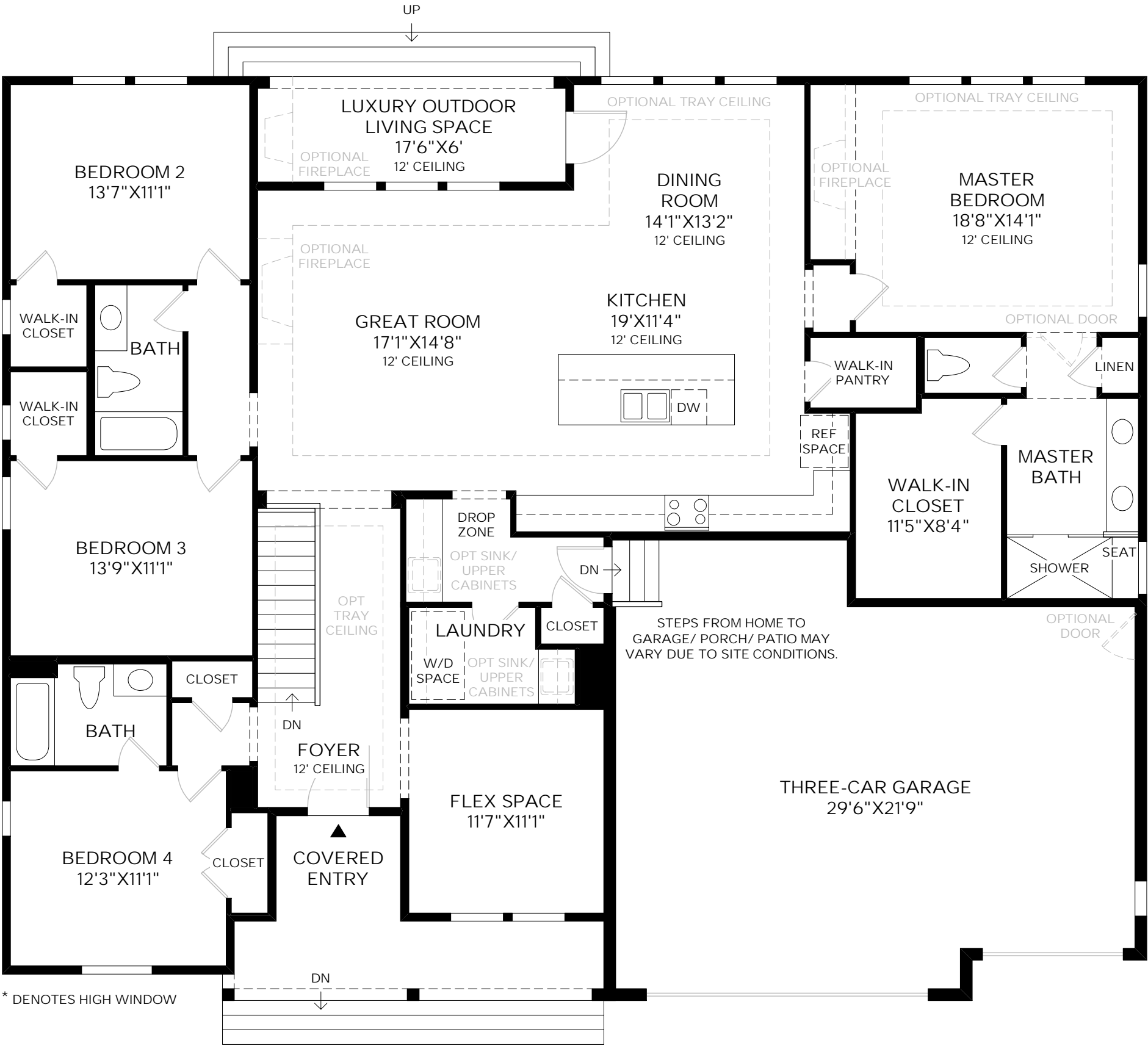
Floor Plan 10' CEILING HEIGHT
