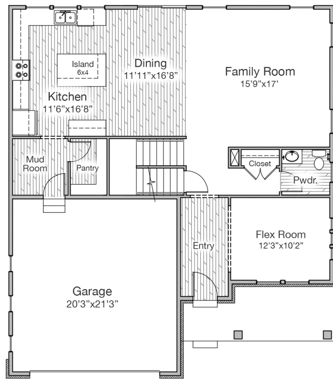
FIRST FLOOR Approx. 1,159 Sq Ft
