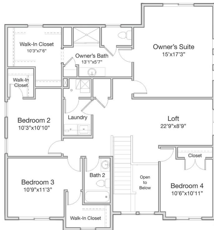
SECOND FLOOR Approx. 1,448 Sq Ft
