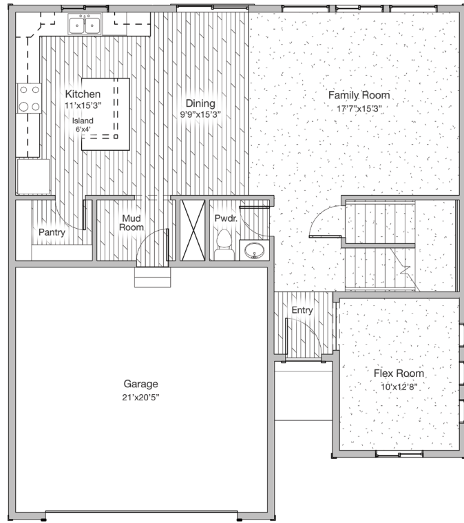
FIRST FLOOR Approx. 1,034 Sq Ft
