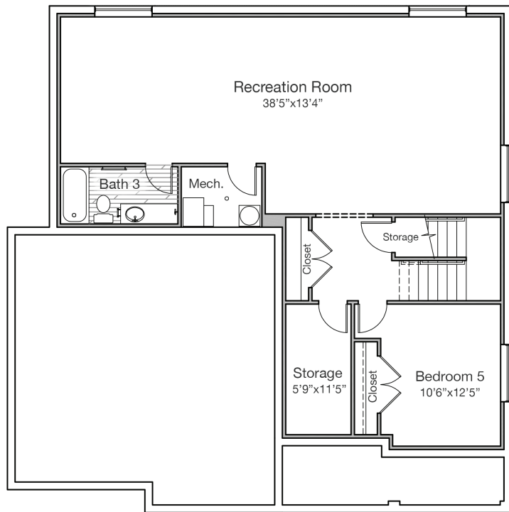
OPTIONAL FINISHED BASEMENT Approx. 1,094 Sq Ft Unfinished
