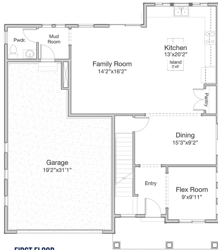
FIRST FLOOR Approx. 995 Sq Ft
