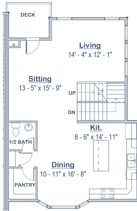
MAIN LEVEL
