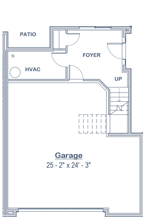
GROUND LEVEL
