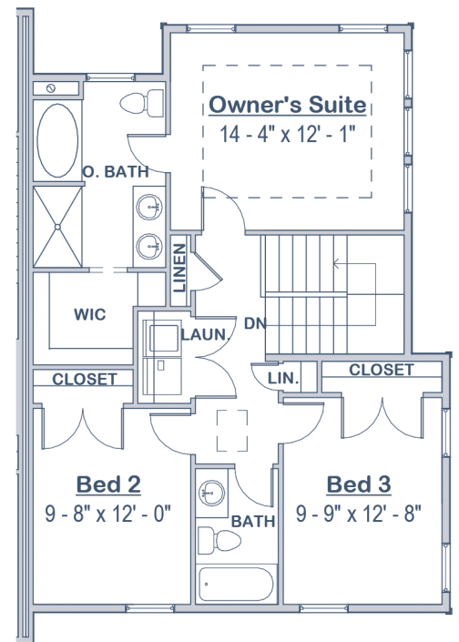
UPPER LEVEL
