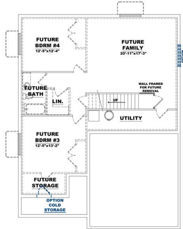
BASEMENT LEVEL
