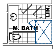
OPTION "A" 60"x42" SHOWER W/ LINEN CLOSET
