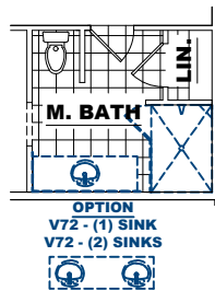
OPTION "A" 60" x 42" SHOWER W/ LINEN CLOSET
