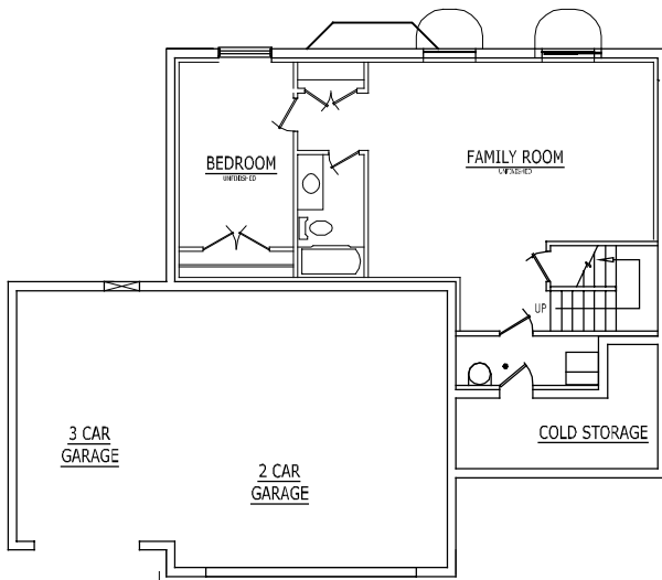
BASEMENT LAYOUT
