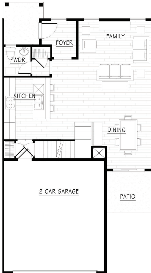
First Floor Approx. 723 sq. ft.
