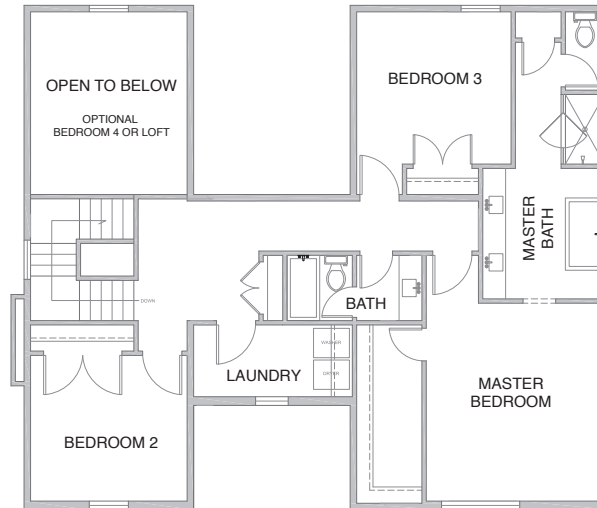
OPTIONAL UPPER FLOOR LAYOUT
