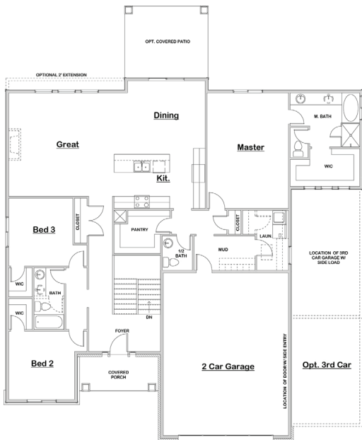
MAIN FLOOR
