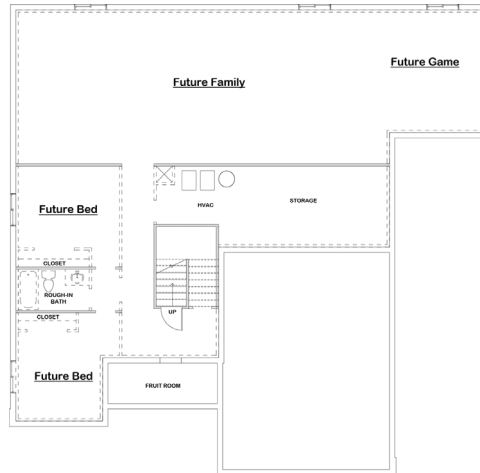
BASEMENT
