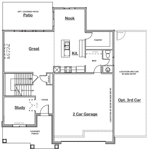
MAIN FLOOR
