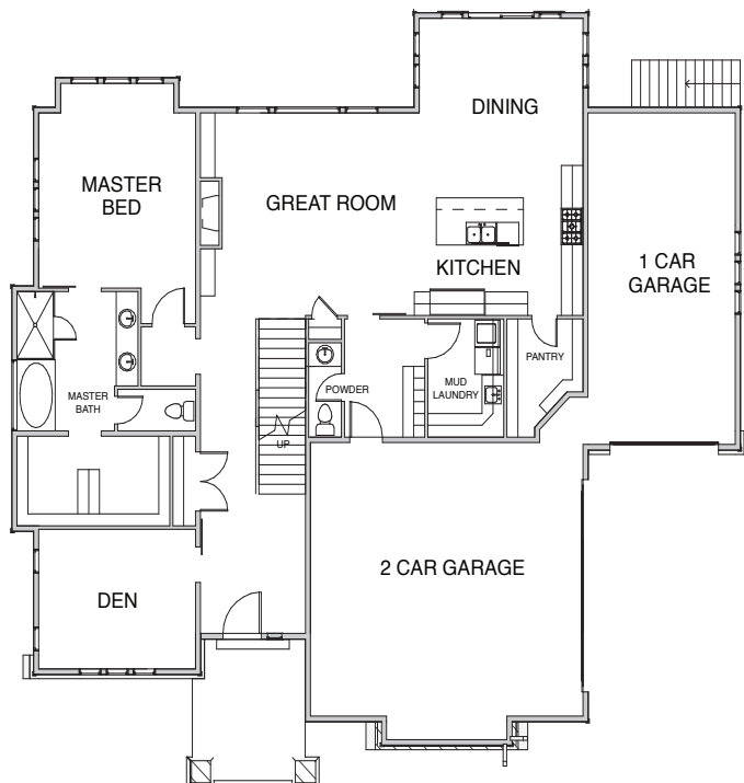
MAIN FLOOR
