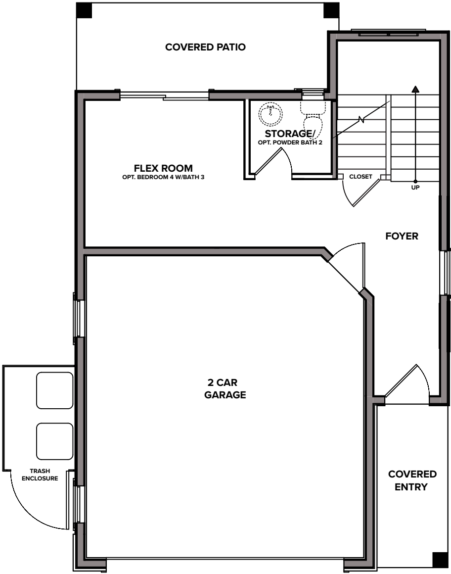
FIRST FLOOR
