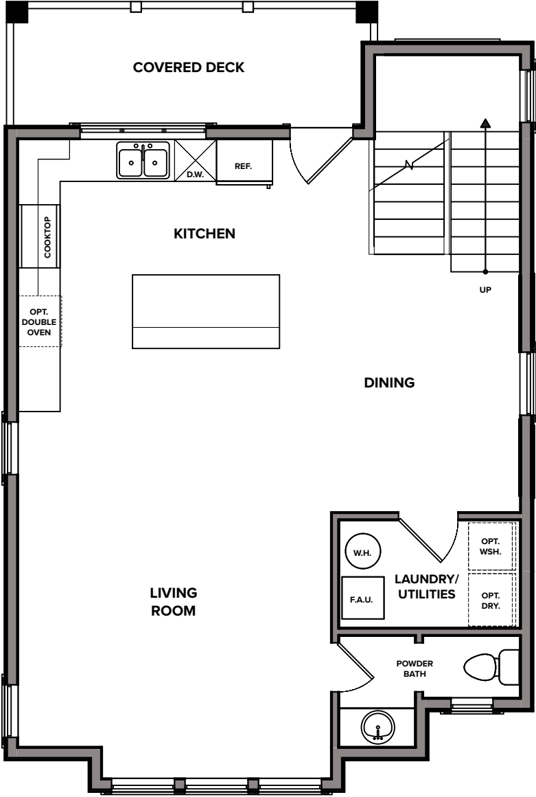
SECOND FLOOR
