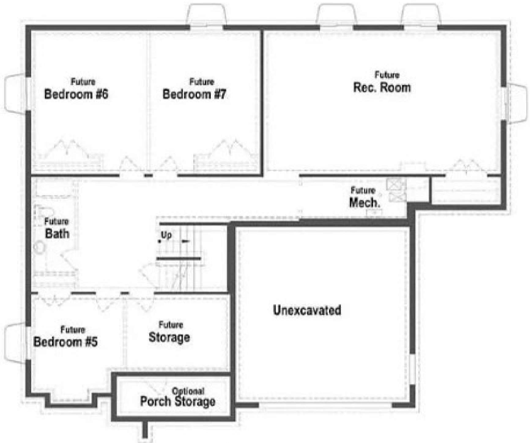
Aaron Basement Floor Plan
