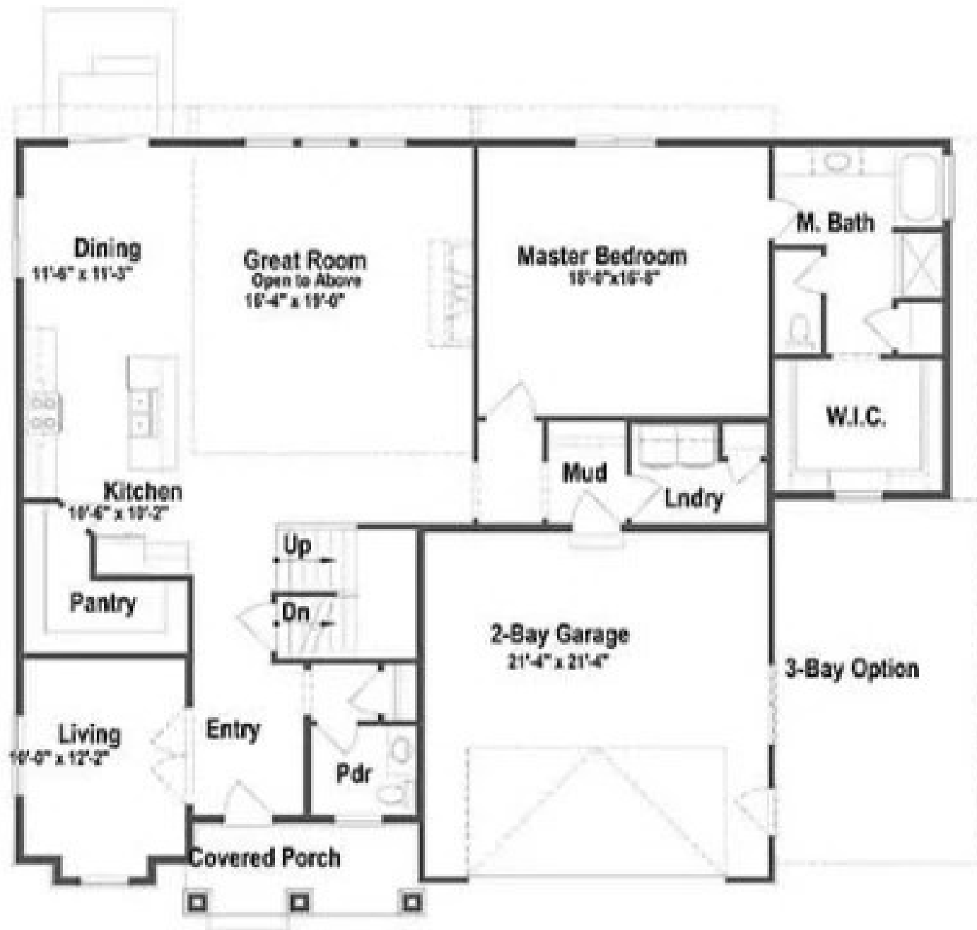
Aaron Main Floor Plan
