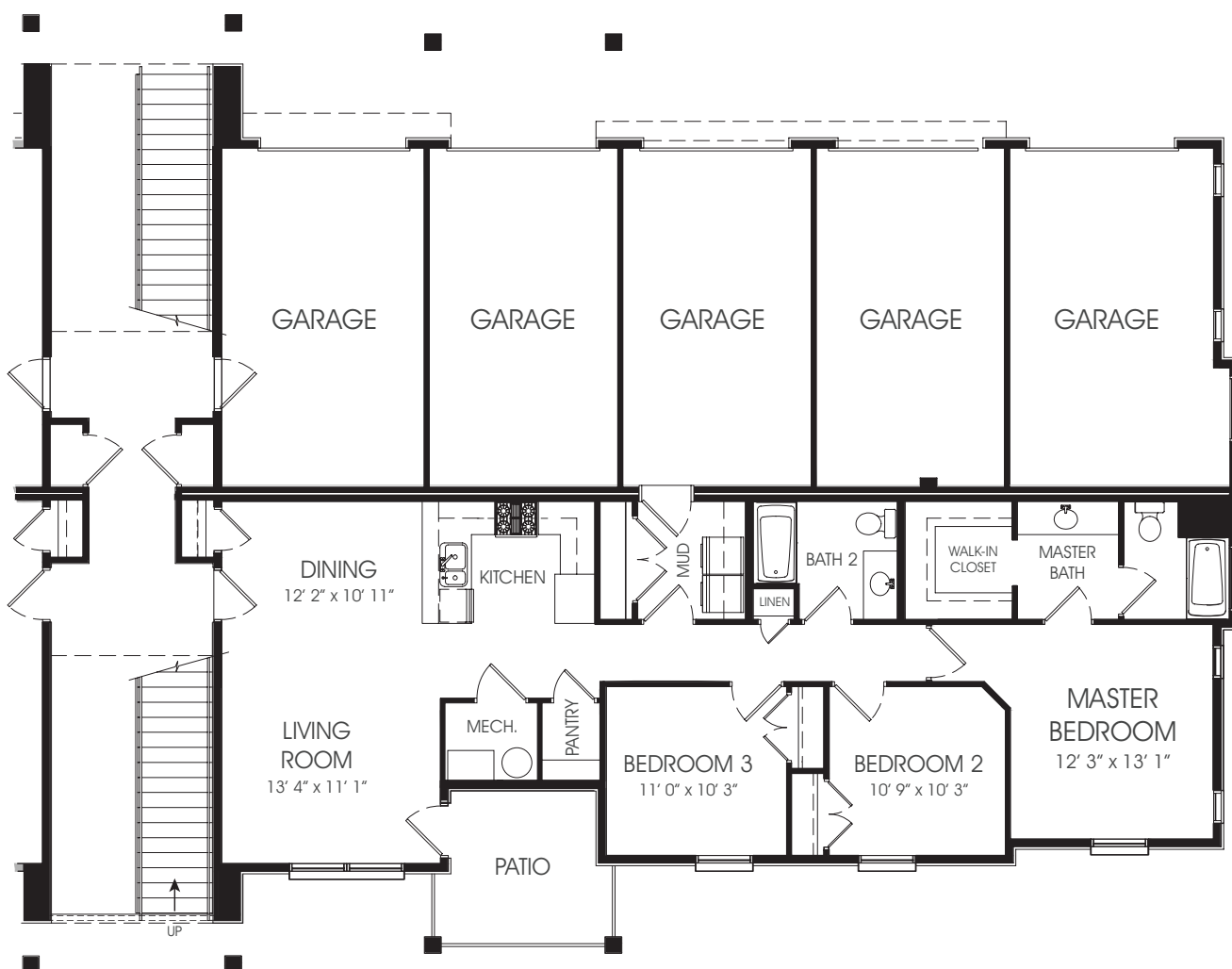
MAIN LEVEL
