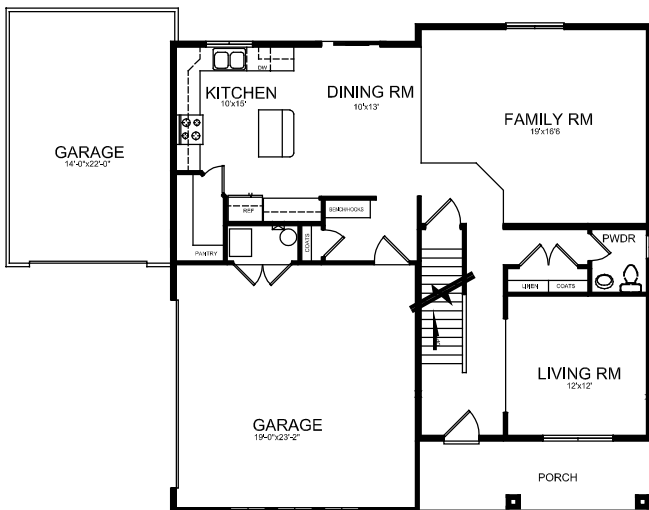
MAIN FLOOR PLAN 1112 S.F.
