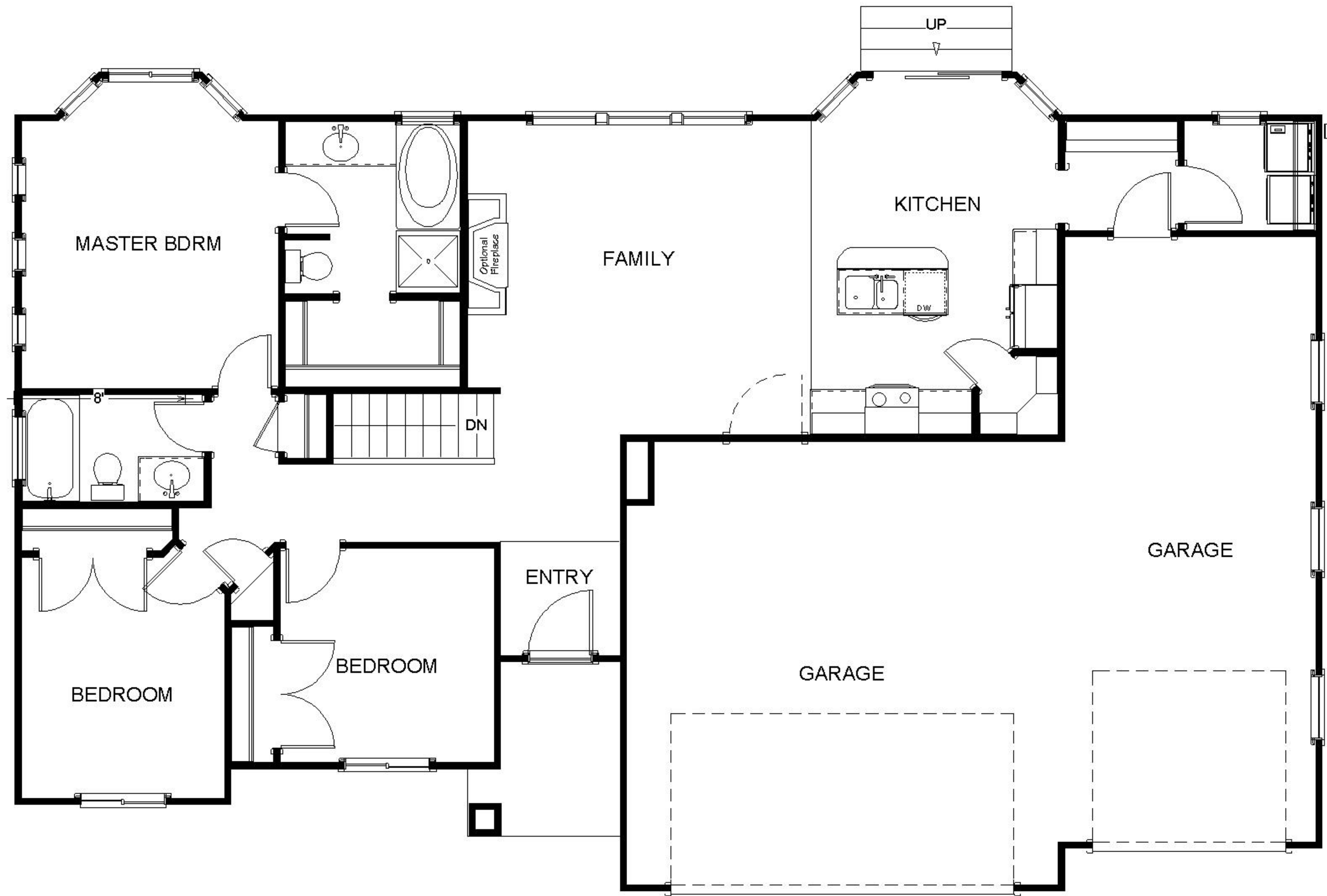
MAIN FLOOR PLAN 1274 SQUARE FEET
