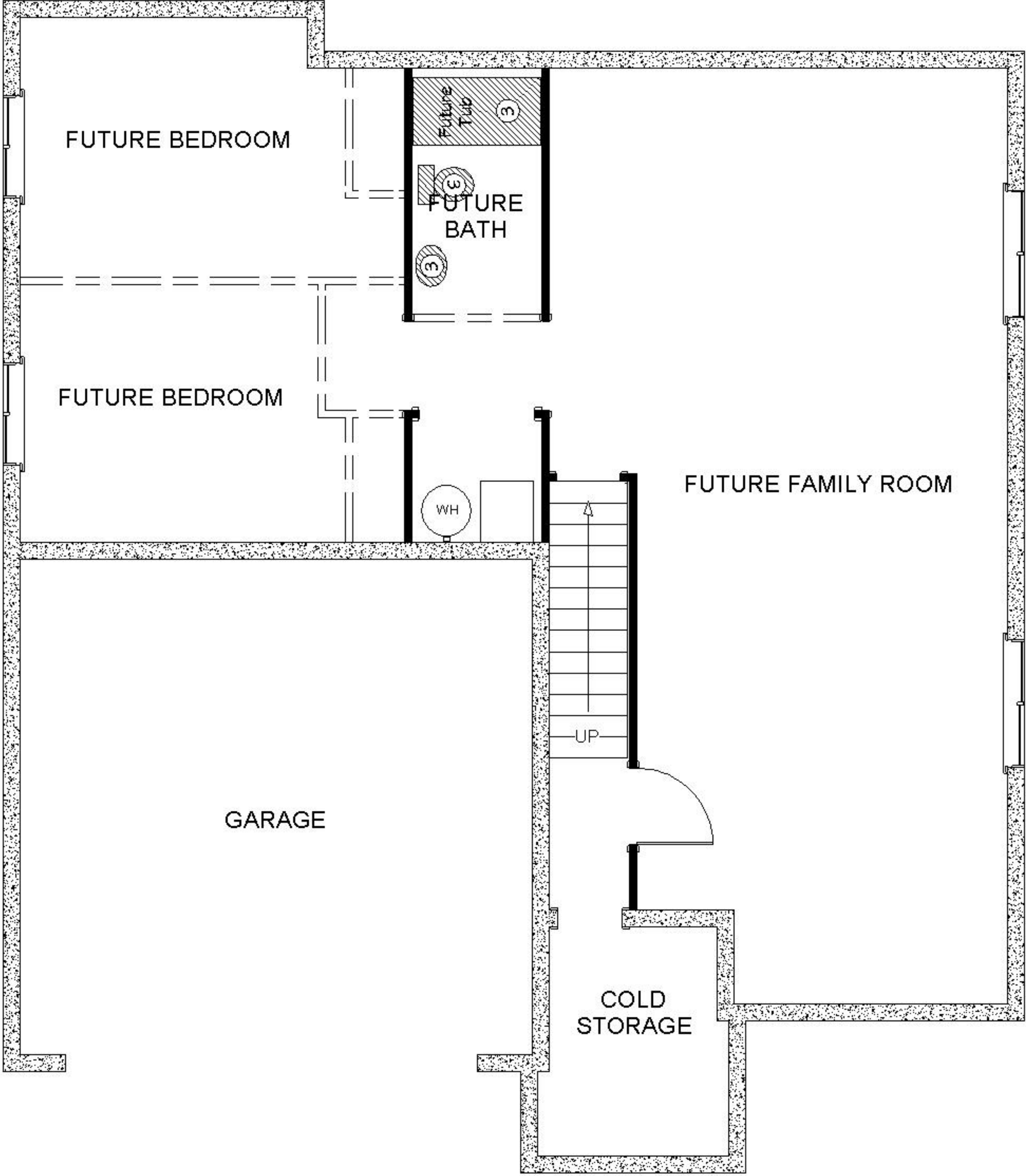
BASEMENT PLAN 1236 SQUARE FEET
