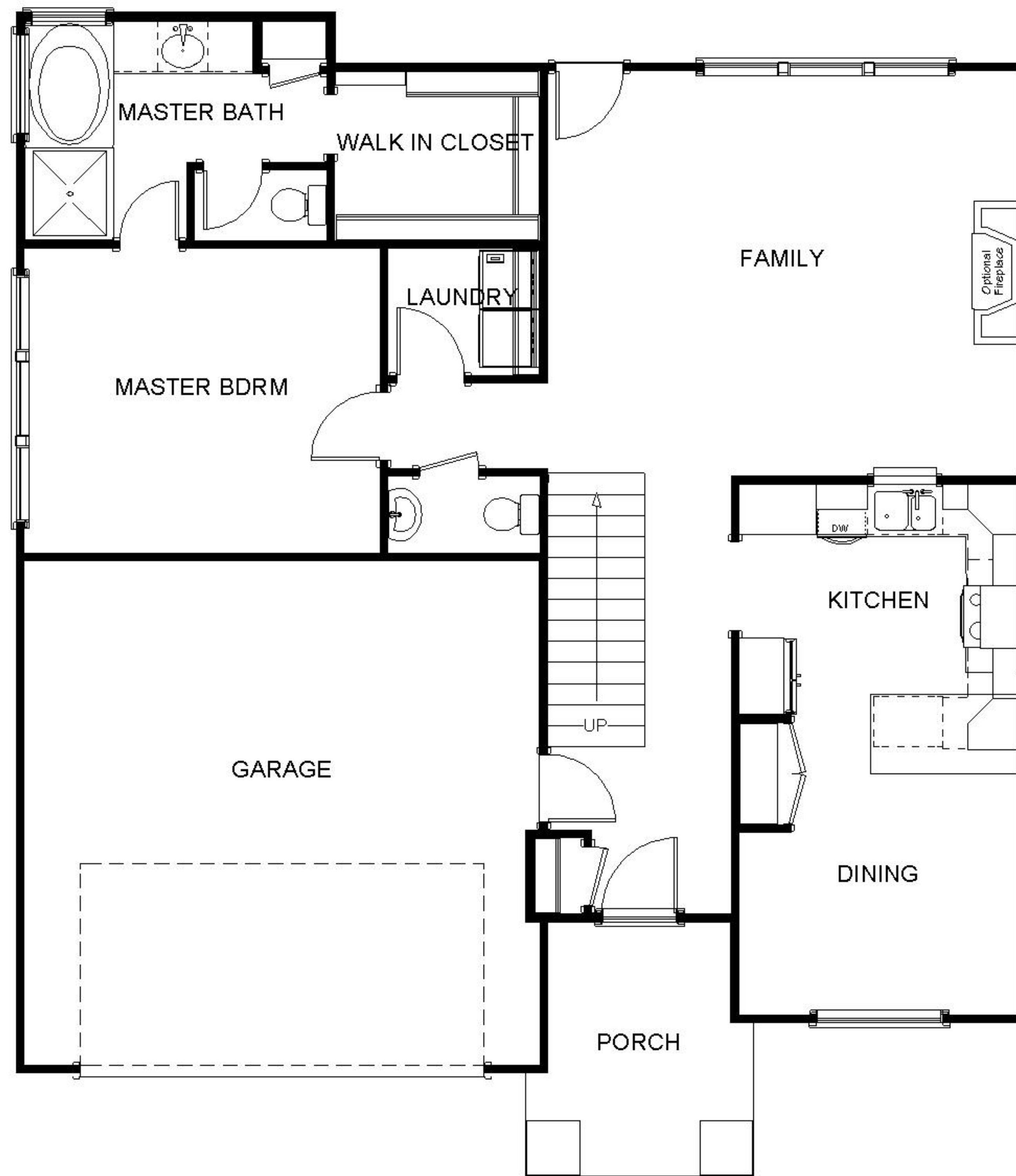
MAIN FLOOR PLAN 1141 SQUARE FEET
