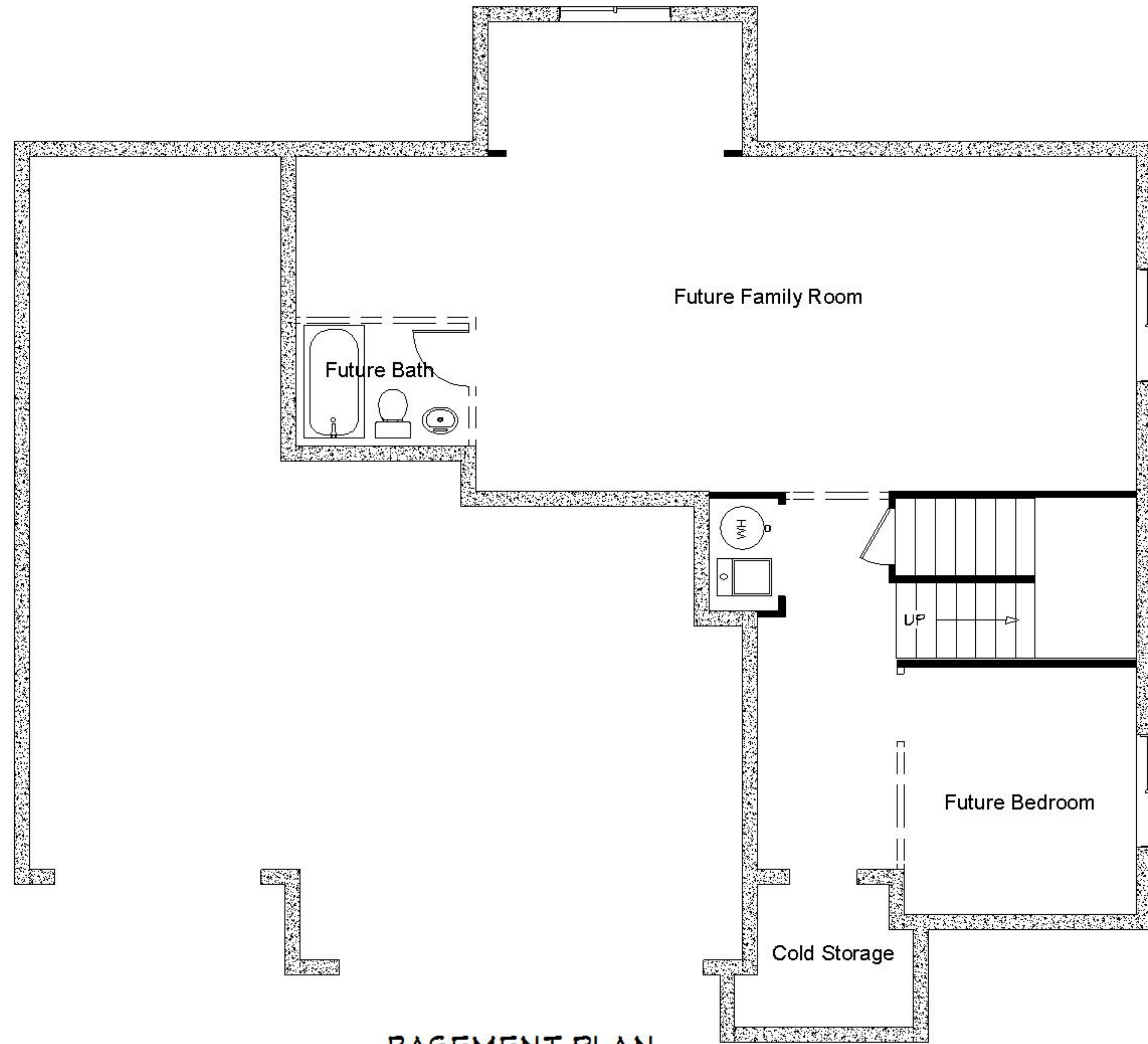
BASEMENT PLAN 1081 Square Feet
