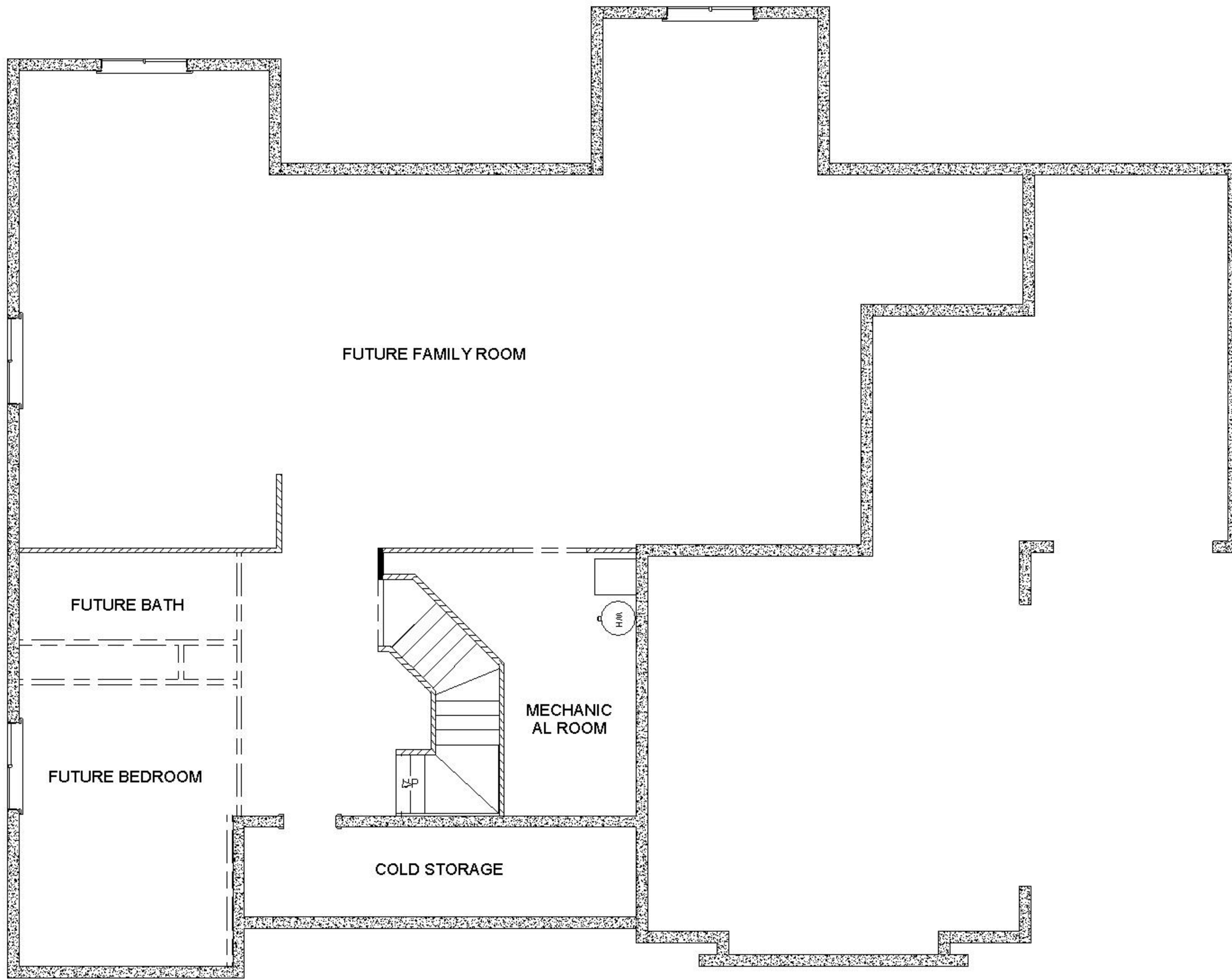
BASEMENT FLOOR PLAN 2247 SQUARE FEET
