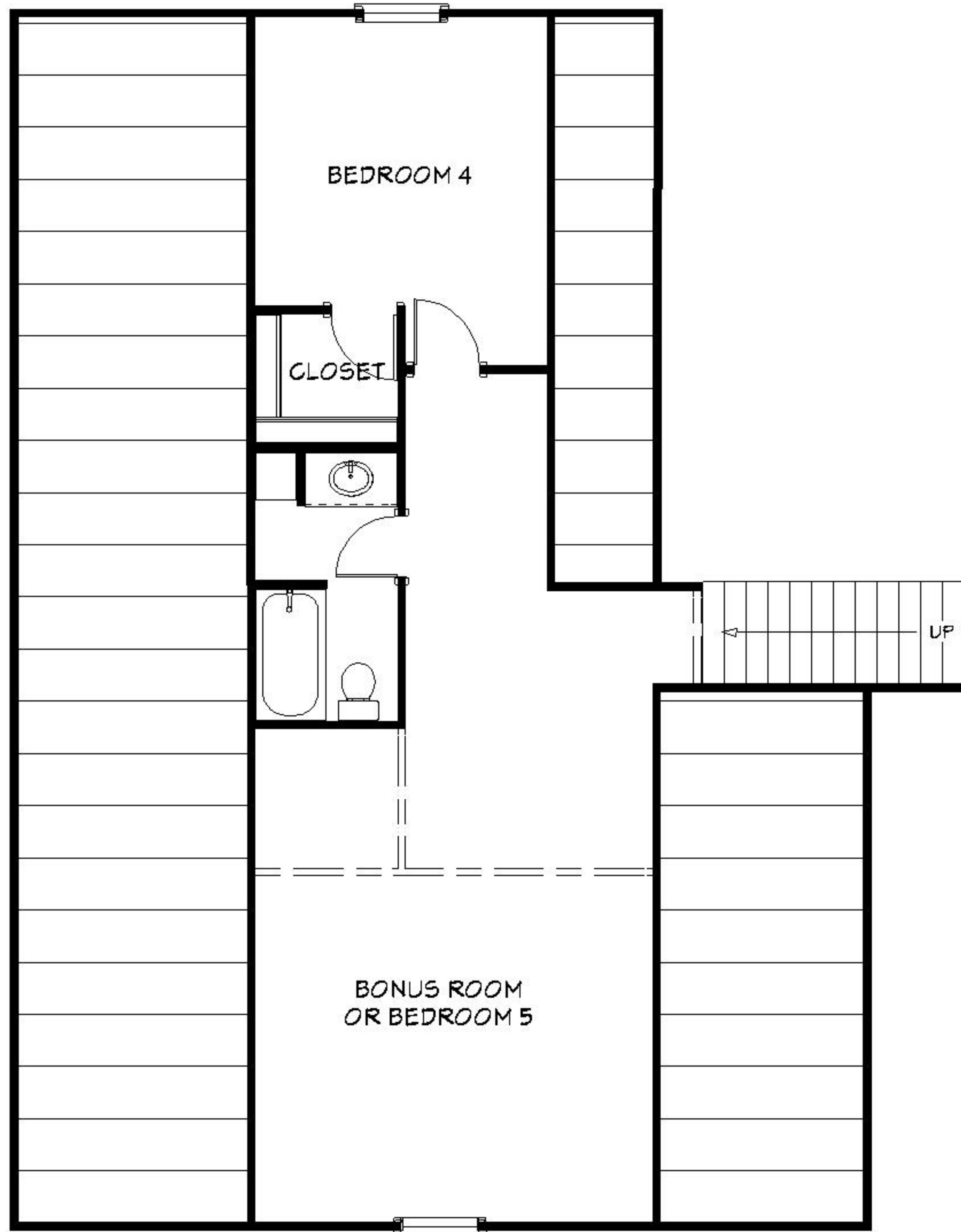
UPPER FLOOR PLAN Upper Floor 662 Square Feet
