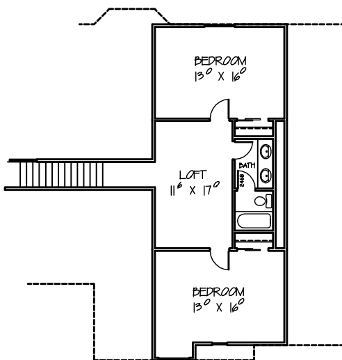
Bonus Room Floor Plan
