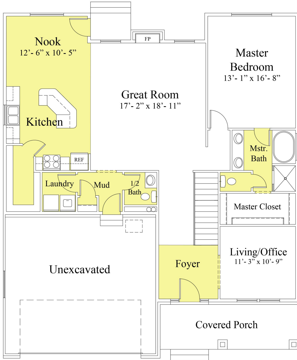
Floor Plan: Washington (R1540) Main Floor
