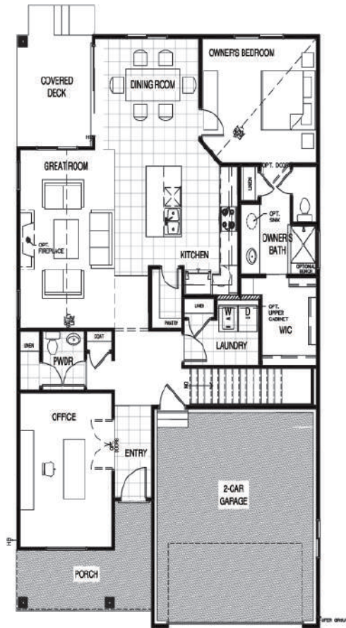
MAIN FLOOR | 1,481 SQ. FT.
