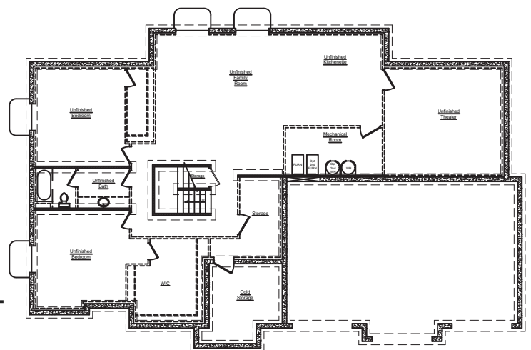
BASEMENT
