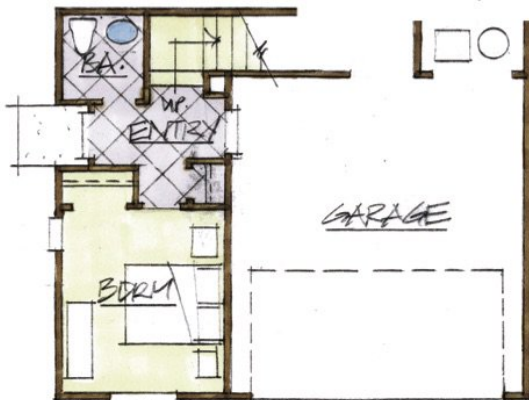
MAIN FLOOR | 313 SQ. FT.
