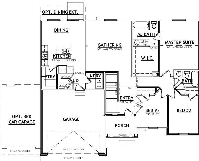
MAIN LEVEL (OPTIONAL 9'-0" CEILING)
