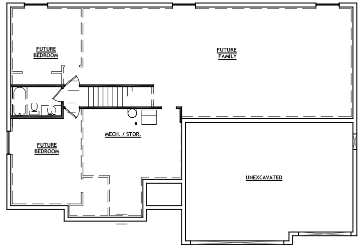
UNFINISHED BASEMENT (OPTIONAL 9'-0" WALLS)
