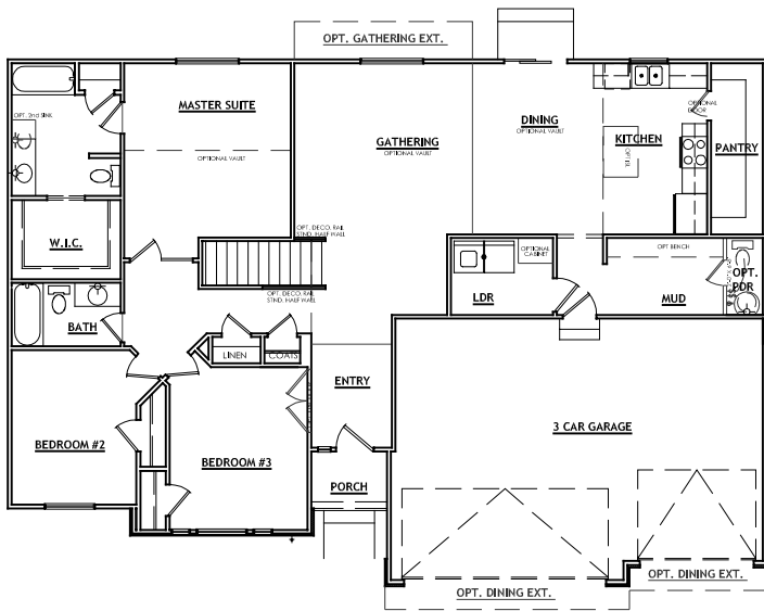
MAIN LEVEL (OPTIONAL 9'-0" CEILING)
