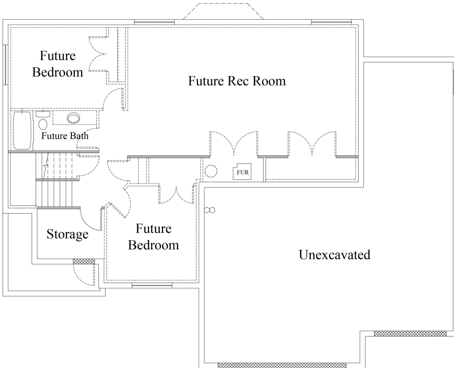
Floor Plan: McKinley (TS2780) Basement
