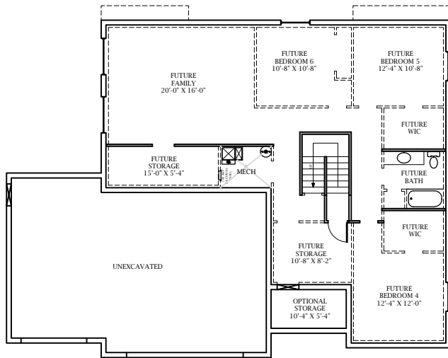
BASEMENT PLAN
