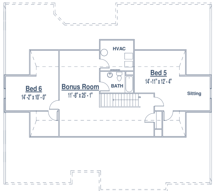
UPPER LEVEL (OPTIONAL LOFT)
