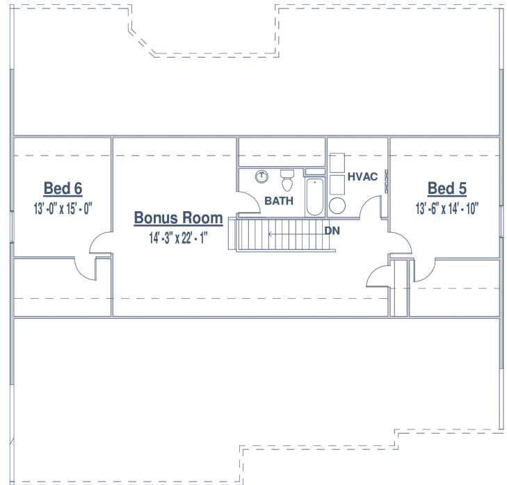
UPPER LEVEL (OPTIONAL LOFT)
