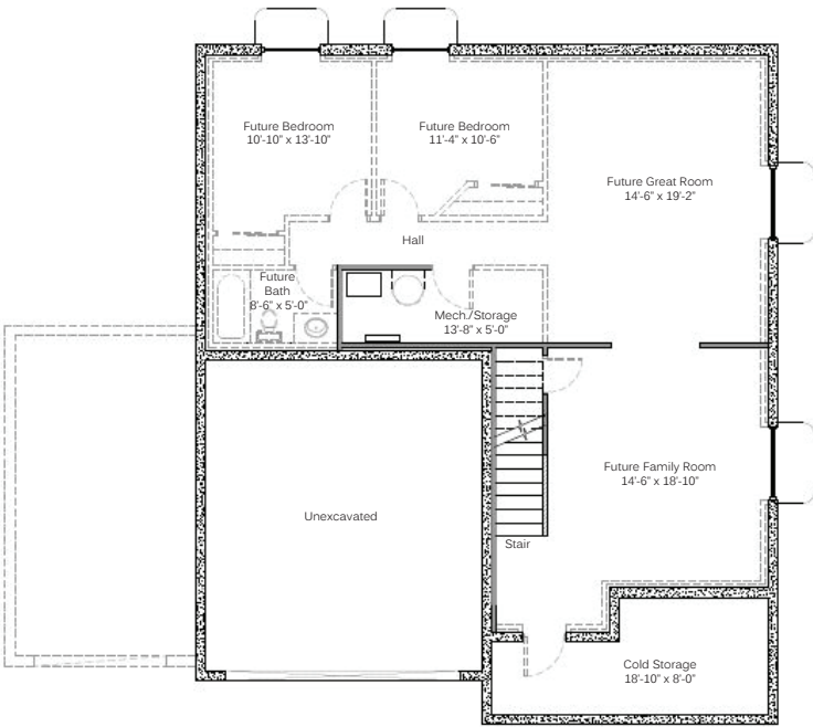
BASEMENT FLOOR
