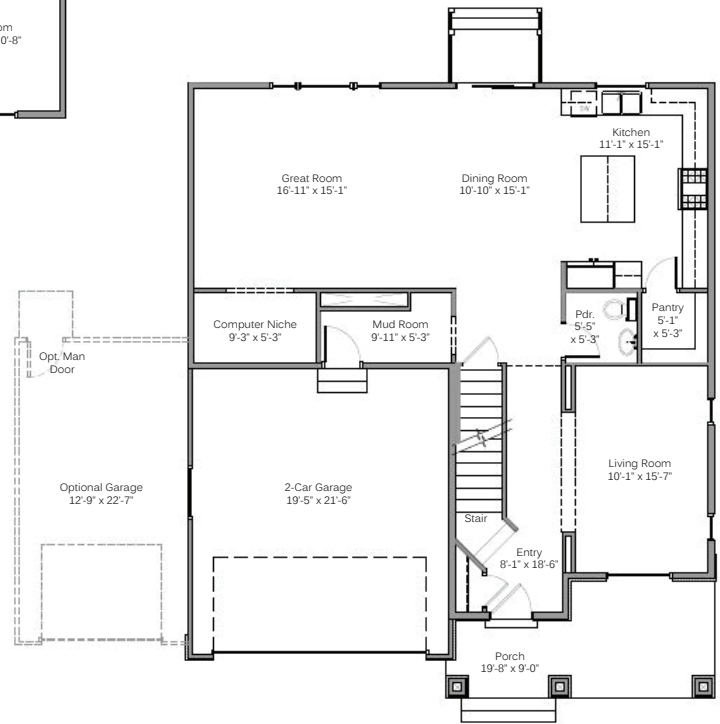
MAIN FLOOR
