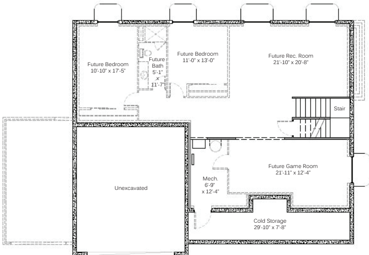
BASEMENT FLOOR
