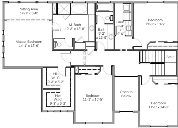
UPPER FLOOR
