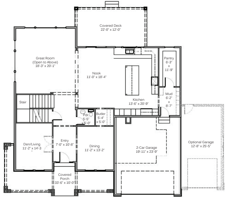
MAIN FLOOR
