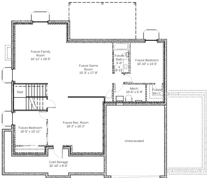
BASEMENT FLOOR
